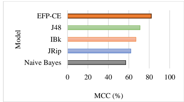
Fig. 7: MCC comparison
