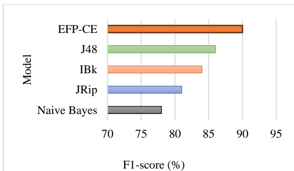
Fig. 6: F1-score comparison
