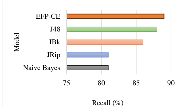
Fig. 5: Recall comparison
