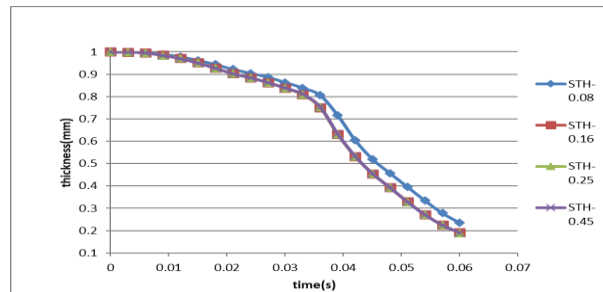
Fig. 13: The trend of thickness reduction of the workpiece sheet at different Friction
