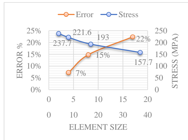
Fig. 6: Solution convergence in on mesh size
