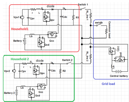
Fig. 2: Electrical model of micro-grid
