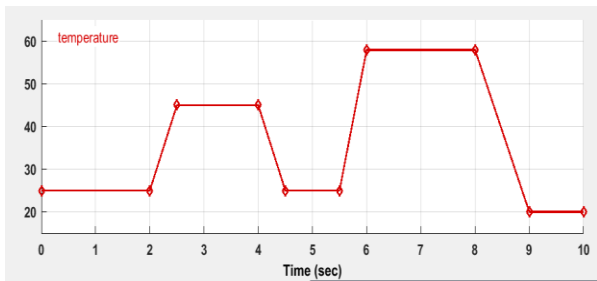
Fig. 10: Profile of temperature
