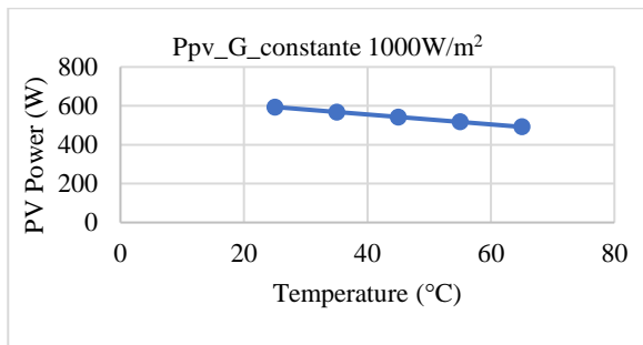
Fig. 14: Variation of PV power with Temperature when irradiance is constant
