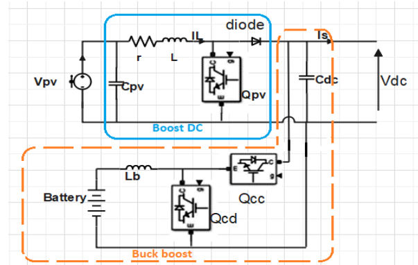
Fig. 3: DC-micro grid system circuit for stability analysis
