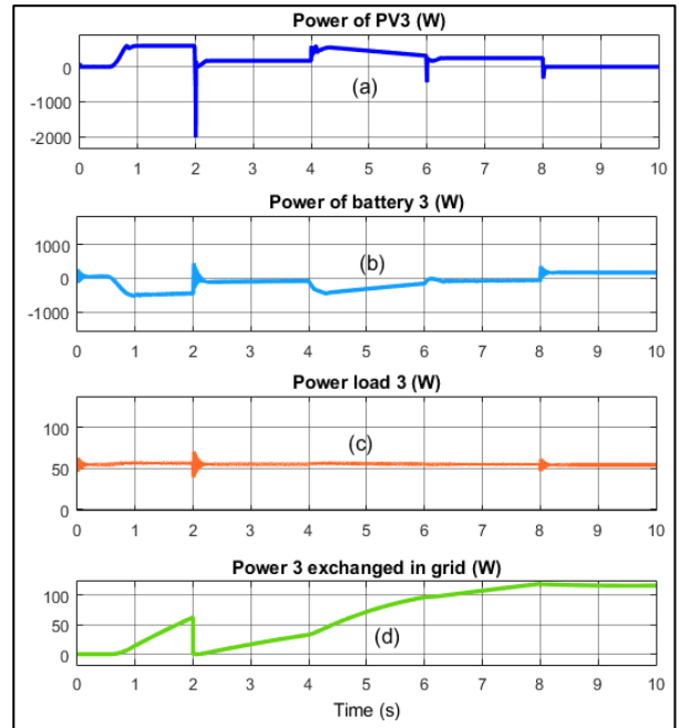
Fig. 24: Characteristics Power of household 3; a: PV power; b: Battery power; c: Load power (W); d: Power 3 exchanged
