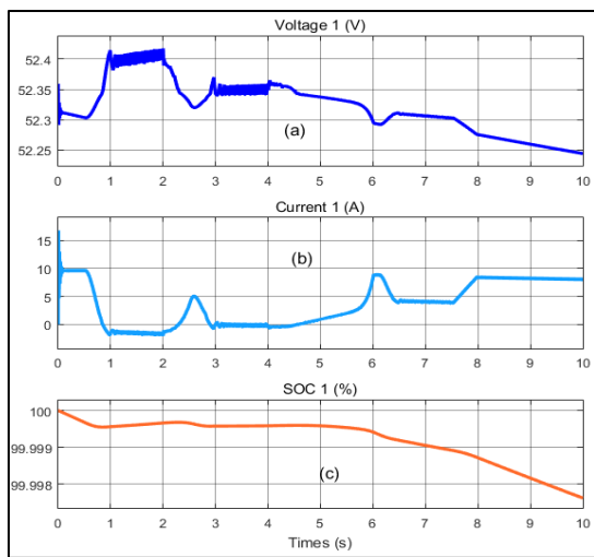
Fig. 18: State of the battery household 1; a: Voltage; b: current; c: State of charge
