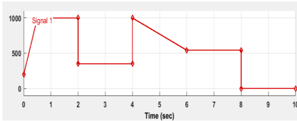
Fig. 9: Profile of irradiance 2
