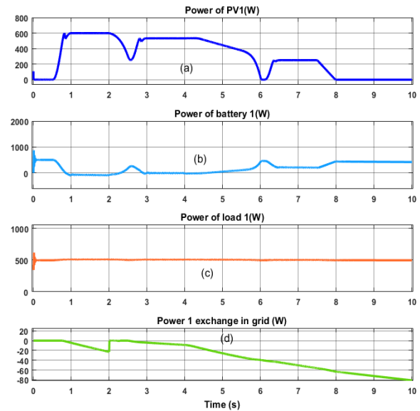
Fig. 11: Characteristics Power of household 1: a: PV power, b: Battery power, c: Load power (W) d: power 1 exchanged
