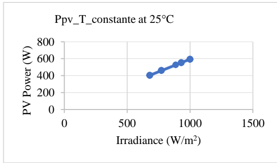
Fig. 13: Variation of PV power with irradiance when Temperature is constant
