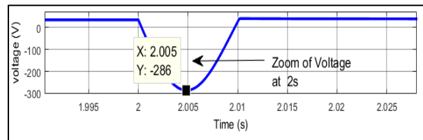
Fig. 17: PV voltage zoom at 2 s of PV2
