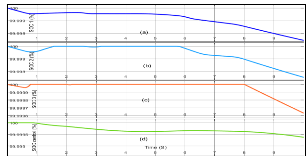
Fig. 28: State of batteries of three households interconnected with central battery with different peak power
