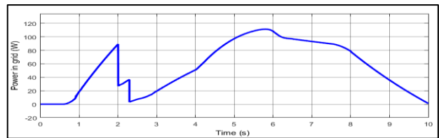
Fig. 27: Power sent in the grid
