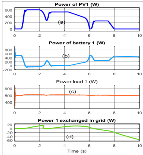
Fig. 22: Characteristics Power of household 1; a: PV power; b: Battery power; c: Load power (W); d: Power 1 exchanged
