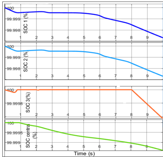
Fig. 25: State of batteries of three households interconnected with central battery with same peak power of 600 Wp
