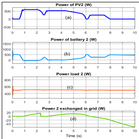
Fig. 23: Characteristics Power of household 2; a: PV power; b: Battery power; c: Load power (W); d: power 2 exchanged
