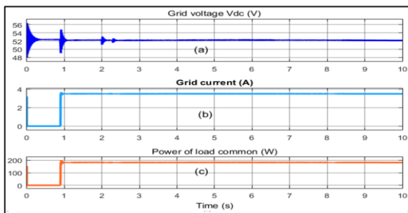
Fig. 26: Grid characteristic; a: Grid voltage; b: Grid current; c: Power of common load
