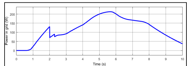
Fig. 29: Power sent in the grid when household 2 has 1200 Wp
