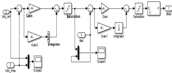
Fig. 4: PI command simulated in Simulink
