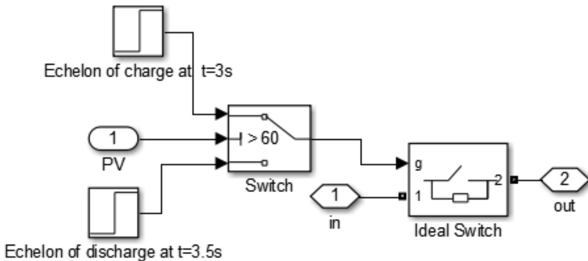
Fig. 6: The interconnect source control process
