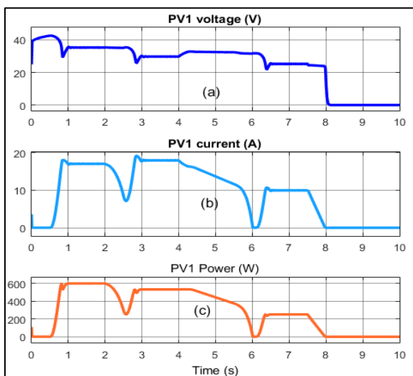
Fig. 15: Characteristics of PV1; a: PV1 Voltage (V); b: PV1 Current (A); c: PV1 power (W)
