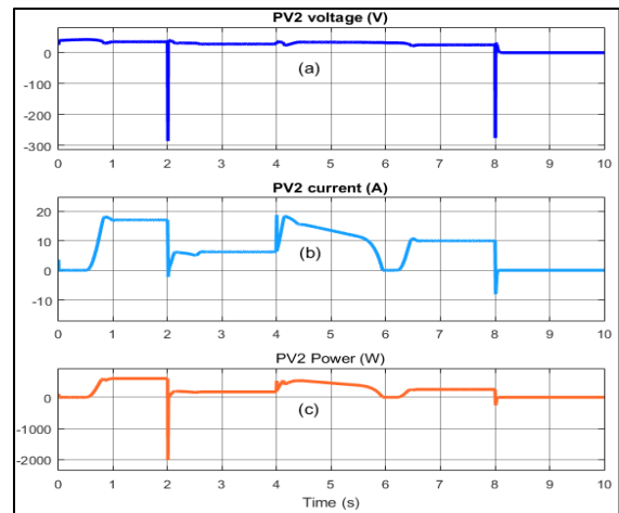
Fig. 16: Characteristics of PV2; a: PV2 Voltage (V); b: PV2 Current (A); c: PV2 power (W)
