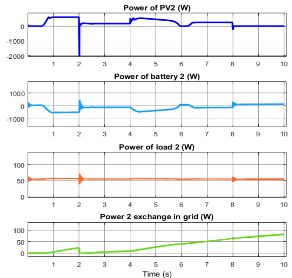
Fig. 12: Characteristics power of household 1: a: PV power, b: Battery power, c: Load power (W); d: Power 2 exchanged
