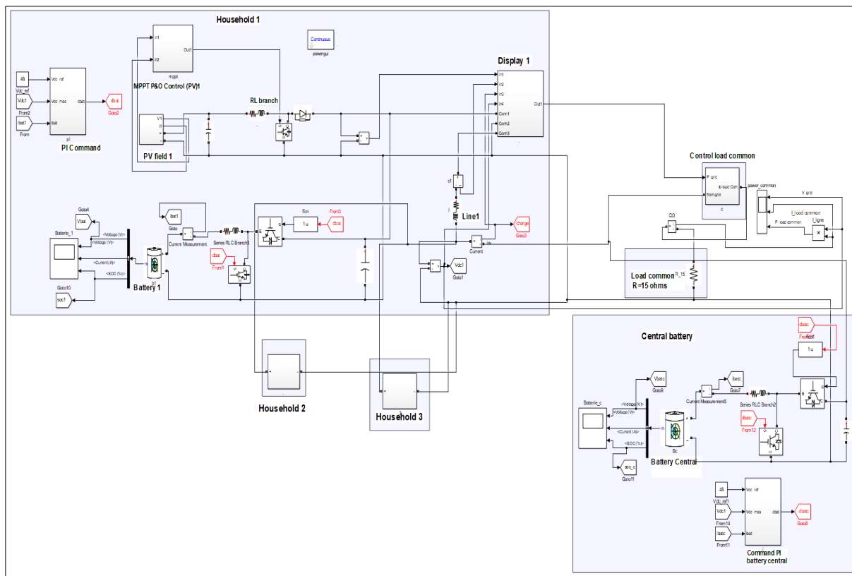
Fig. 7: Scheme of the microgrid with PI command in Matlab Simulink R2016a
