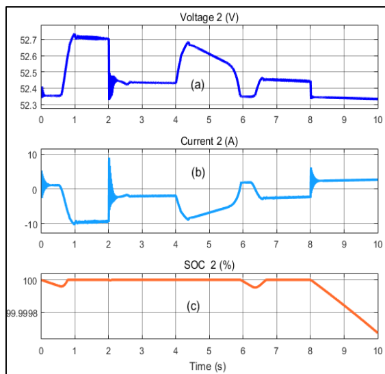
Fig. 19: State of the battery household 2; a: Voltage; b: current; c: State of charge
